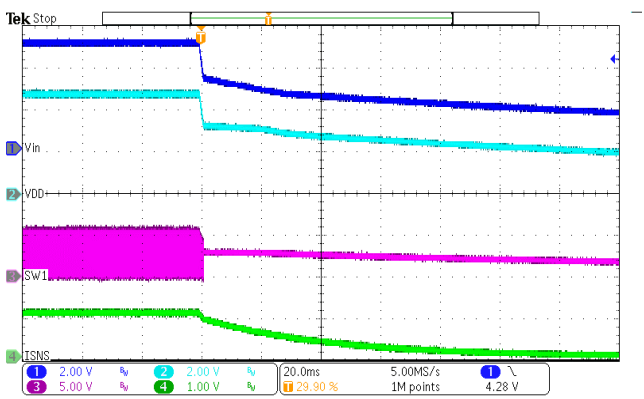
Figure 11. Power Down
