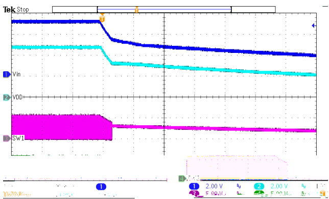
Figure 9. Power Down
