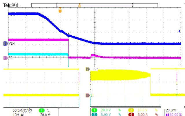
Figure 9. Power Down (CH-1: Vin, CH-2: Vout, CH-3: PG, CH-4: IL)
