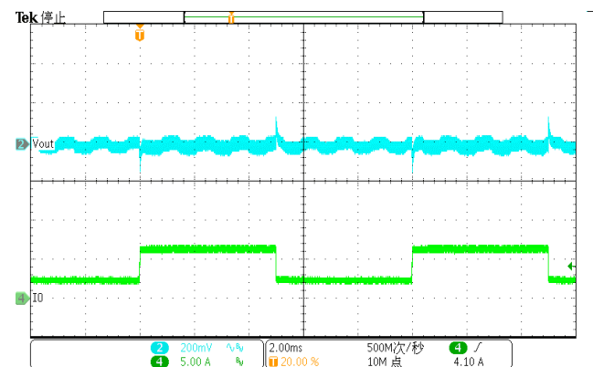
Figure 12. Load Transient (2A-6A, SR=1600mA/us, CH-1: Iout, CH-2: Vout)
